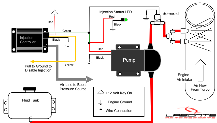
Typical System Install
